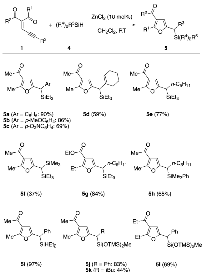
Scheme 4. Zinc(II)-catalyzed synthesis of furan derivatives 5 from carbonyl enyne derivatives 1 and silanes 4 . Reaction conditions: 1 (0.2 mmol), 4 (6 equiv), \text{ZnCl}_2 (10 mol%), \text{CH}_2\text{Cl}_2 (0.1 M), RT. Values in parentheses are the yields of the isolated products.
